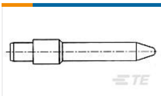
TE 产品编号445287-1 POST,GUIDE/GROUND,HDI,LOGIC
