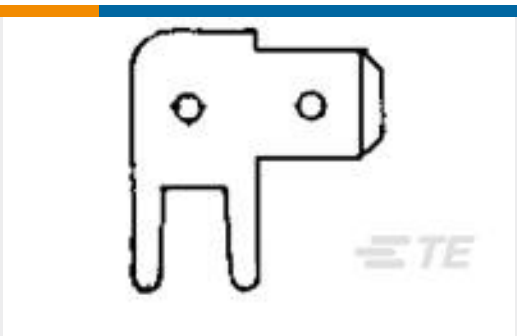
TE 产品编号1-726389-2 187 FASTON,FLAG,TAB,TPBR
