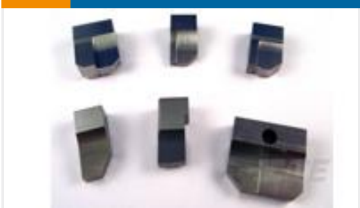
TE 产品编号2-1333218-6 ANVIL, END FEED (.100)
