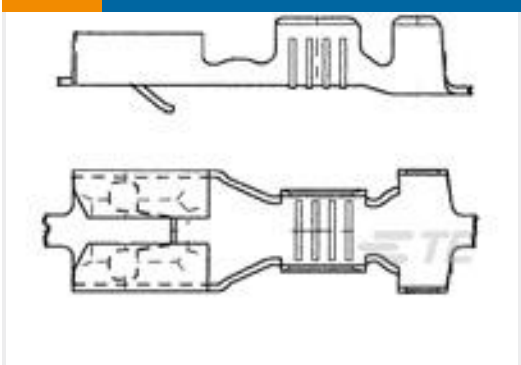
TE 产品编号282180-1 FF 187 REC 0.5-1.5MM2 TPBR
