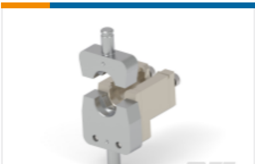
TE 产品编号2234183-1 DIE SET DIA 3.6MM F 50MM2
