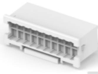
TE 产品编号2-2323743-0 HOUSING, PLUG, GWT, 20P, DUAL ROW, EP2.5
