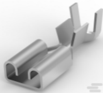
TE 产品编号2232975-1 187 FASTON,REC.,20-16 AWG,TPBR
