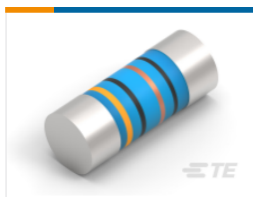
TE 产品编号2-2176314-0 MELF SMA_A 3K9 0.1% 15PPM 0102 0.3W
