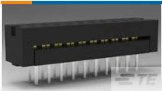
TE 产品编号1-746610-4 16 DIP PLUG, 100CL, LEAD FREE
