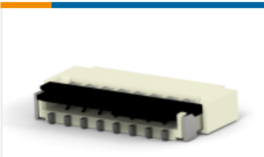
TE 产品编号1-2328724-5 15PIN 0.3MMP FPC CONNECTOR, FRONT FLIP
