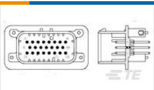
TE 产品编号1-776228-2 HEADER ASSY, 23 POS VERTICAL
