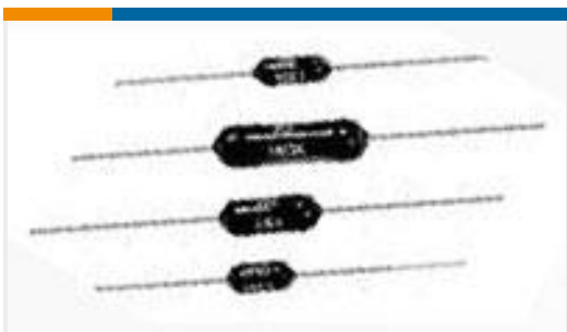
TE 产品编号 1879639-1 H4P 10R 0.5% 50PPM
