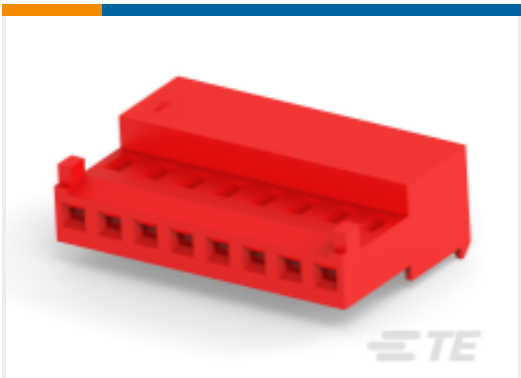
TE 产品编号3-644020-3 Nylon Gold Plated Receptacle: 2.54 mm, With Mating Alignment, MTA 100
