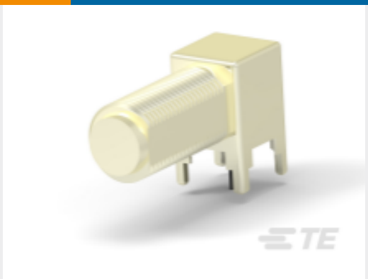
TE 产品编号5-1634540-1 F Type Connector: Male (Jack), Right-Angle, Elbow Jack PCB, 75 Ohm
