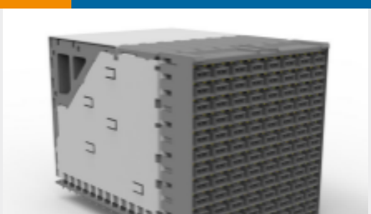
TE 产品编号2187576-1 SW PIR RECT, 100OHM, 12X8
