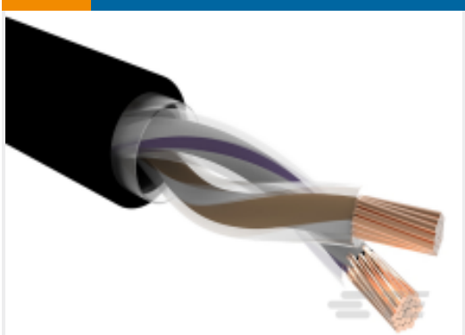
TE 产品编号2460793001 ACW5229-0.75-12/92-0
