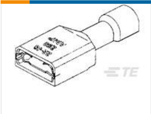
TE 产品编号2-520263-2 ULTRA-FAST 250 ASY REC 22-18 TPBR
