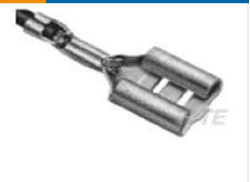
TE 产品编号1742594-1 205 FASTON,REC.,18-14 AWG,NPST
