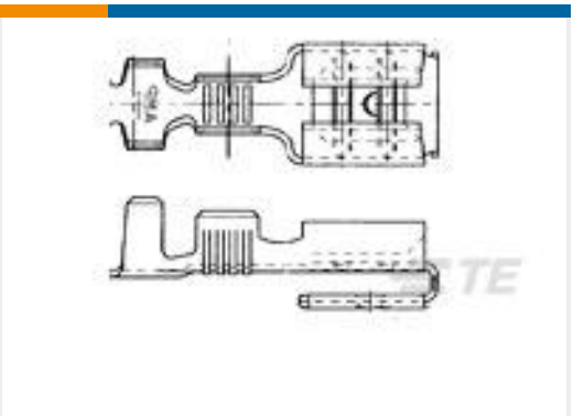
TE 产品编号160739-1 250 FASTON, PIGGYBACK REC., 18-14 AWG, BR
