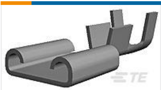
TE 产品编号1-160301-6 250 FASTON, REC., 10-12 AWG, TPBR
