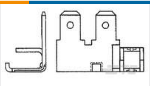
TE 产品编号444069-2 TERM BOARD INS DISPL 4.8 TAB 20-18 NL
