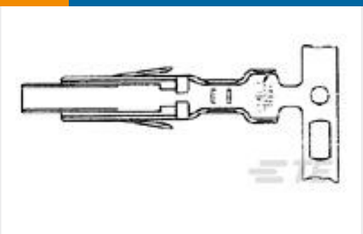
TE 产品编号170312-1 POWER CONN.CONTACT
