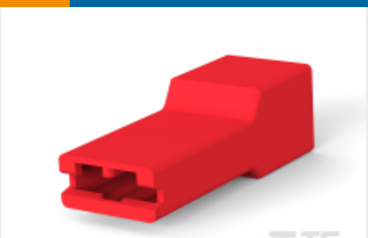
TE 产品编号171706-2 FASTON 250 INS POD NYLON RED
