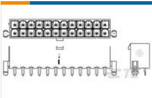
TE 产品编号1-2029265-0 10P VAL-U-LOK VRTHDR W/PGS GW
