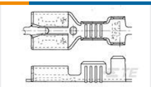
TE 产品编号100605-7 250 FASTON, REC., 14-17AWG, TPS
