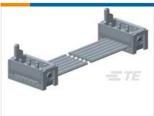
TE 产品编号1483351-3 MICRO-MATCH LEAD 06P 250MM
