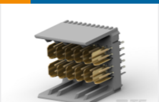
TE 产品编号2274610-1 HM-ZD 2PR HDR 24P 2.5MM
