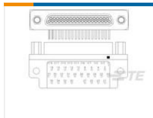
TE 产品编号1532255-4 M83513/10-F01NP = MCKS-N1-P-37PRT1
