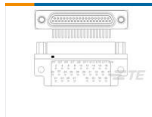
TE 产品编号1532263-1 M83513/13-F01CN = MCKS-C2-B-37SRT1
