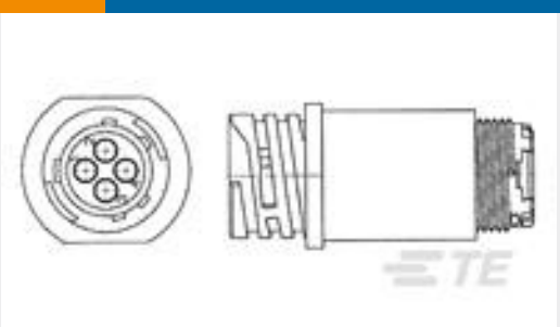
TE 产品编号1977877-1 SLD CPC RCPT ASSY, 11-4, STD SEX, UV RESIST
