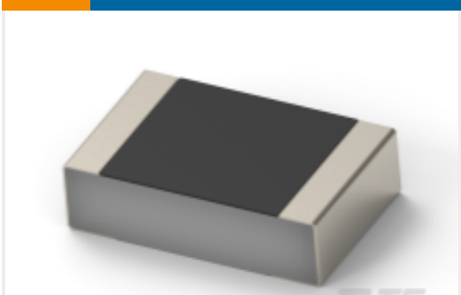
TE 产品编号7-2176074-4 CPF 0201 33K2 0.5% 50PPM 1K RL
