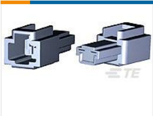
TE 产品编号1-172127-1 FF 250 REC HSG 1P NYLON NAT
