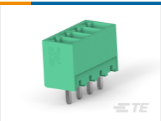
TE 产品编号1-2351886-6 16POS TB HDR 180 DEG, PITCH 3.5, TL3.4mm
