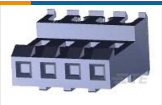
TE 产品编号3-640600-4 04P MTA156 CONN ASSY 20AWG LF
