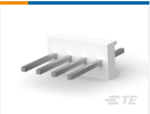
TE 产品编号1-640456-8 Polyester Vertical PCB Header: 2.54 mm, Unshrouded, No Mating Alignment
