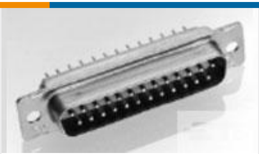
TE 产品编号204502-4 RECEPT ASSY,26 POSN,AMPLIMITE
