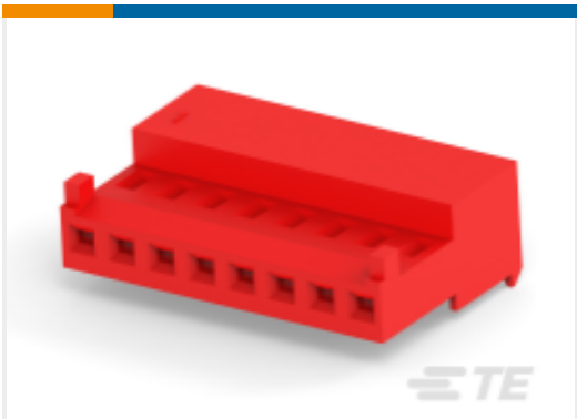
TE 产品编号4-647477-2 Nylon Gold Plated Receptacle: 2.54 mm, With Mating Alignment, MTA 100
