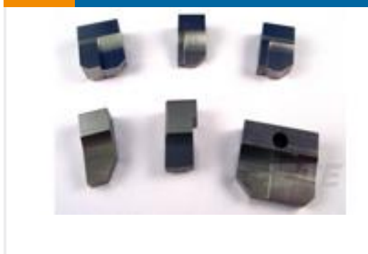
TE 产品编号2-1333229-2 ANVIL, COMBINATION SPECIAL
