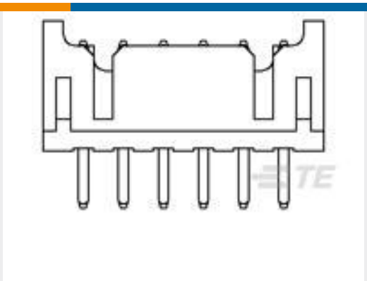
TE 产品编号1-1470109-0 2.0mm Pitch Header,Dip 10p
