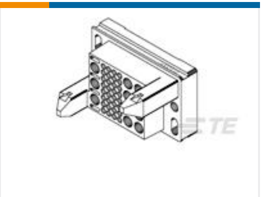
TE 产品编号194242-1 AMP POWER HOUSING, PLUG, 43 POS
