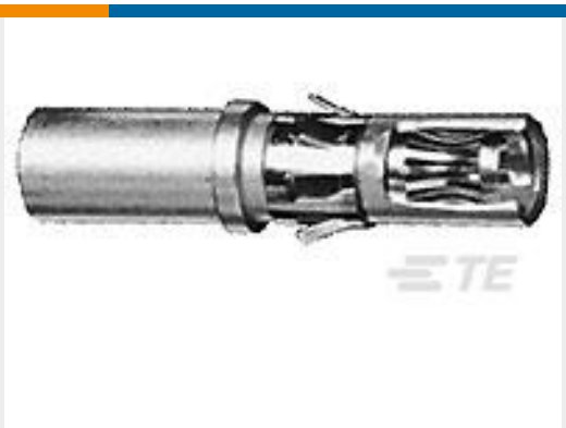
TE 产品编号193535-1 SKT ASSY., POWER, #12-14 AWG
