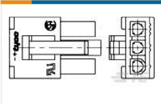
TE 产品编号1586027-4 4P SR RCPT VAL-U-LOK V0
