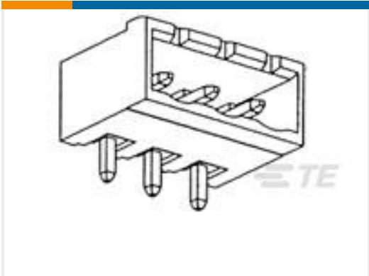
TE 产品编号1-796644-2 12POS 5.0MM CE R/A HDR,TRM BLK
