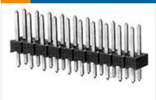
TE 产品编号103240-5 10 MOD II HDR DRST B/A .100CL
