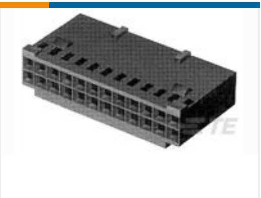
TE 产品编号2-87631-9 34 MODIV HSG COMP DR .100 POL
