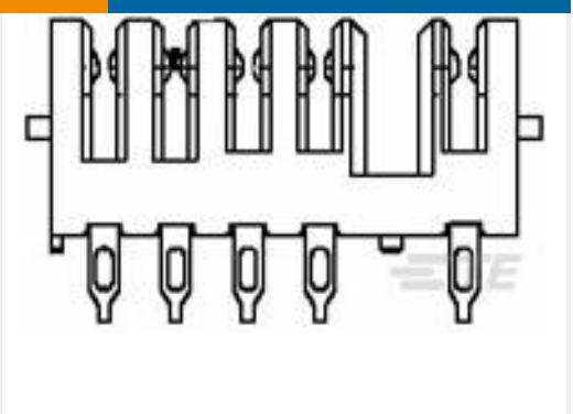
TE 产品编号1473969-1 REC ASS'Y FOR 2.5 SLIM BATTERY
