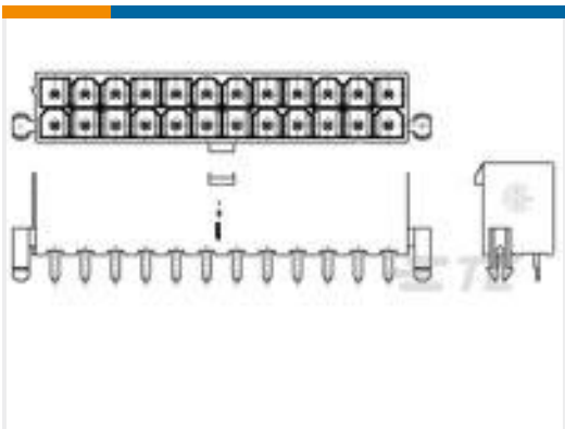
TE 产品编号1-1586039-2 12P VAL-U-LOK VRT HDR W/P V2
