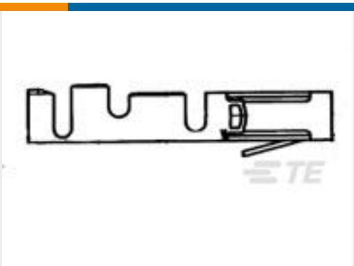
TE 产品编号182207-2 AMP MODU II RCPT CONT COSI LP
