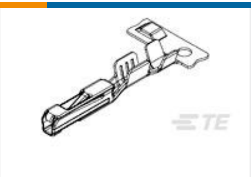
TE 产品编号1326028-2 0.64MM FEMALE CONTACT,AU, 22AWG
