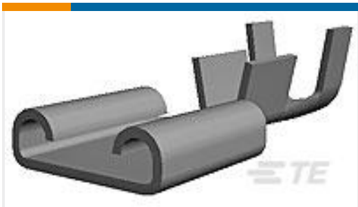
TE 产品编号170179-1 205 FASTON,REC.,18-14 AWG,BR
