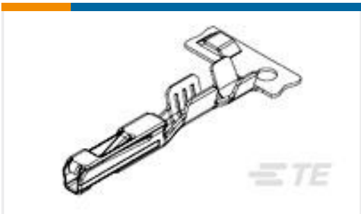
TE 产品编号1326028-2 0.64MM FEMALE CONTACT,AU, 22AWG
