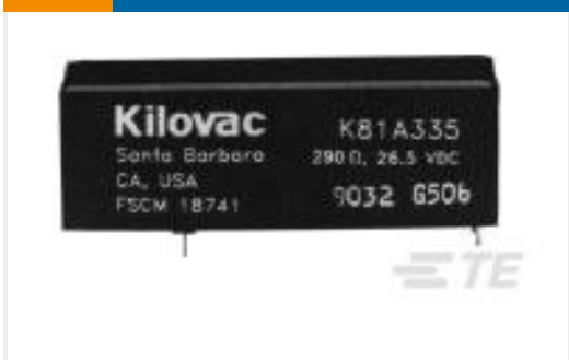
TE 产品编号1618241-5 K81A235=RELAY, VACUUM, SPST-NO
