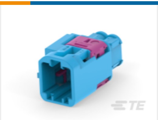
TE 产品编号2-2298724-3 4POS,MATE-AX,PIN HSG ASSY, 180DEG,COD C
