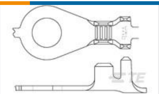
TE 产品编号444151-2 RING TONGUE 2.5-4.0 MM2 0.81 ELECTROPBR
